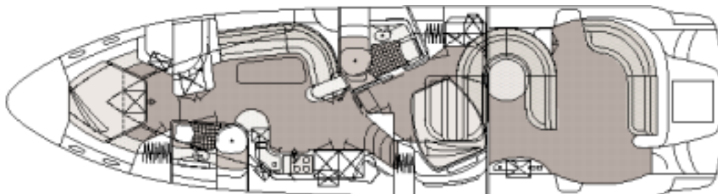
Cabin Layout w/Cockpit Seating
