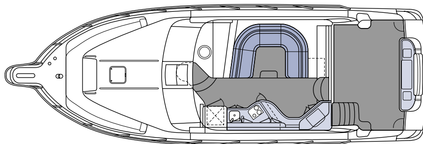
Upper Cabin / Cockpit Layout
